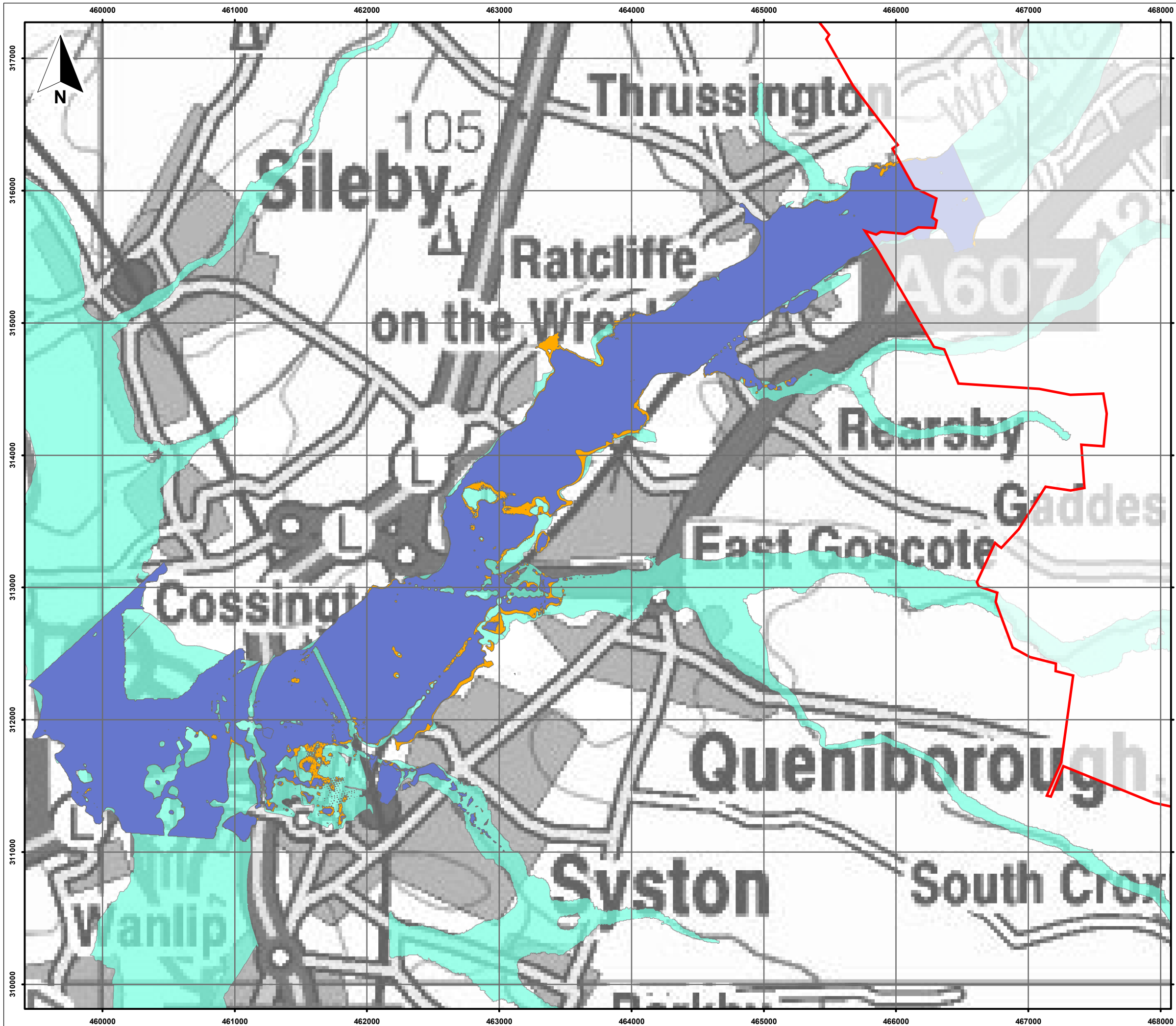
Figure 4.11 River Wreake - Comparison of extents of modelled Flood Zone 3a and Flood Zone 3a + climate change
