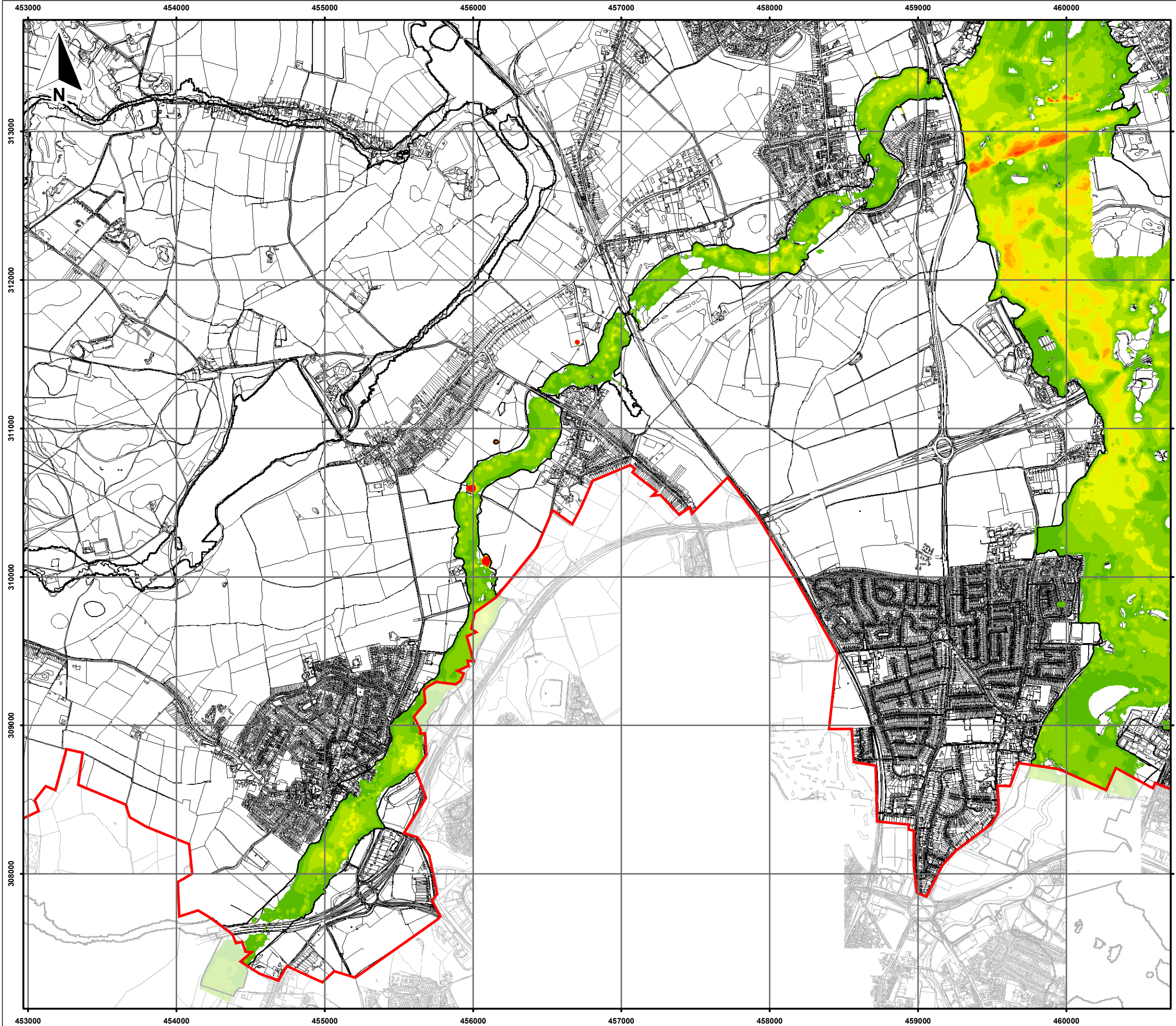
Figure 4.14 Rothley Brook - Flood Depth during 1% (1 in 100 flood)
