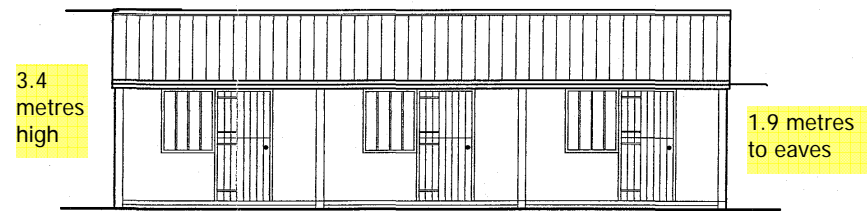
FRONT ELEVATION
