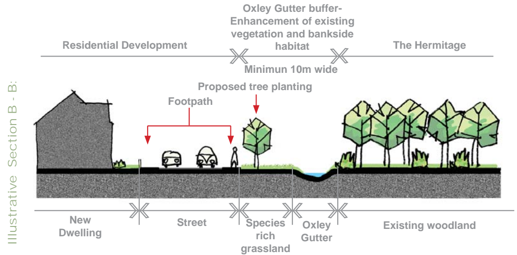
Illustrative Section through Oxley Gutter by the Hermitage
