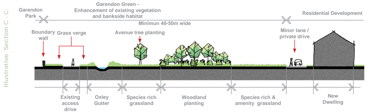
Illustrative Section of Green Infrastructure Corridor adjacent to Garendon Park
