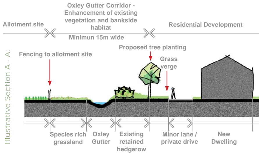
Illustrative Section through Oxley Gutter to the south of Bunker Hill
